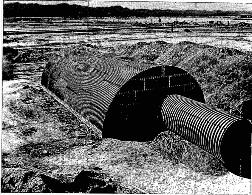
Fig. 1—Building 3.6 without earth cover.
